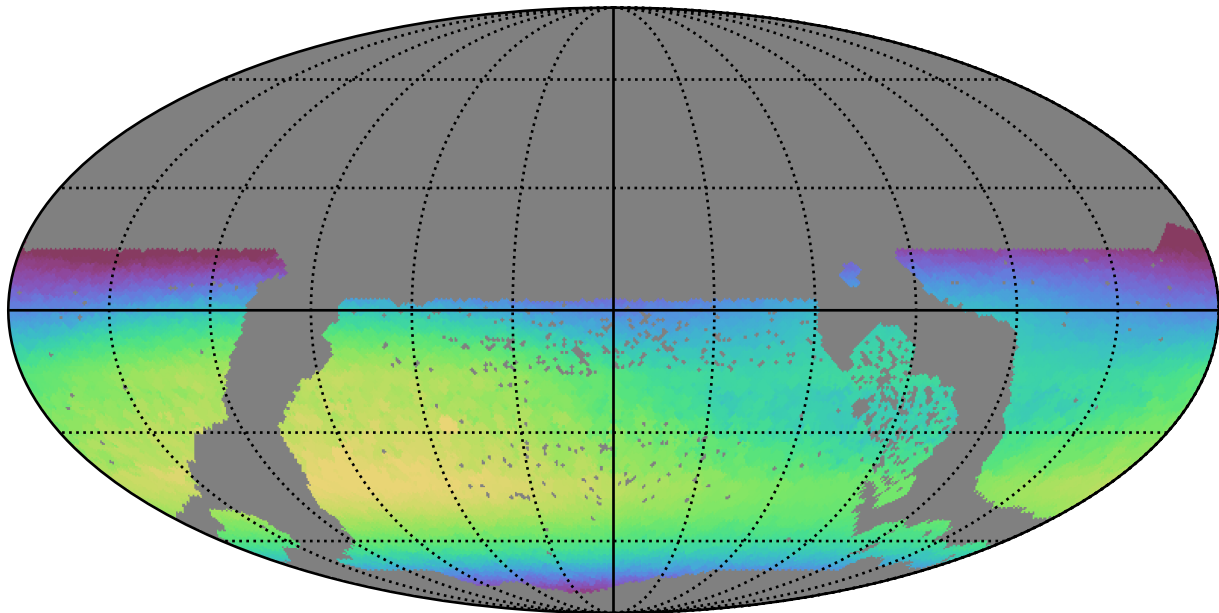
too_100_4v3.4_10yrs WFD i band: Max skyBrightness
