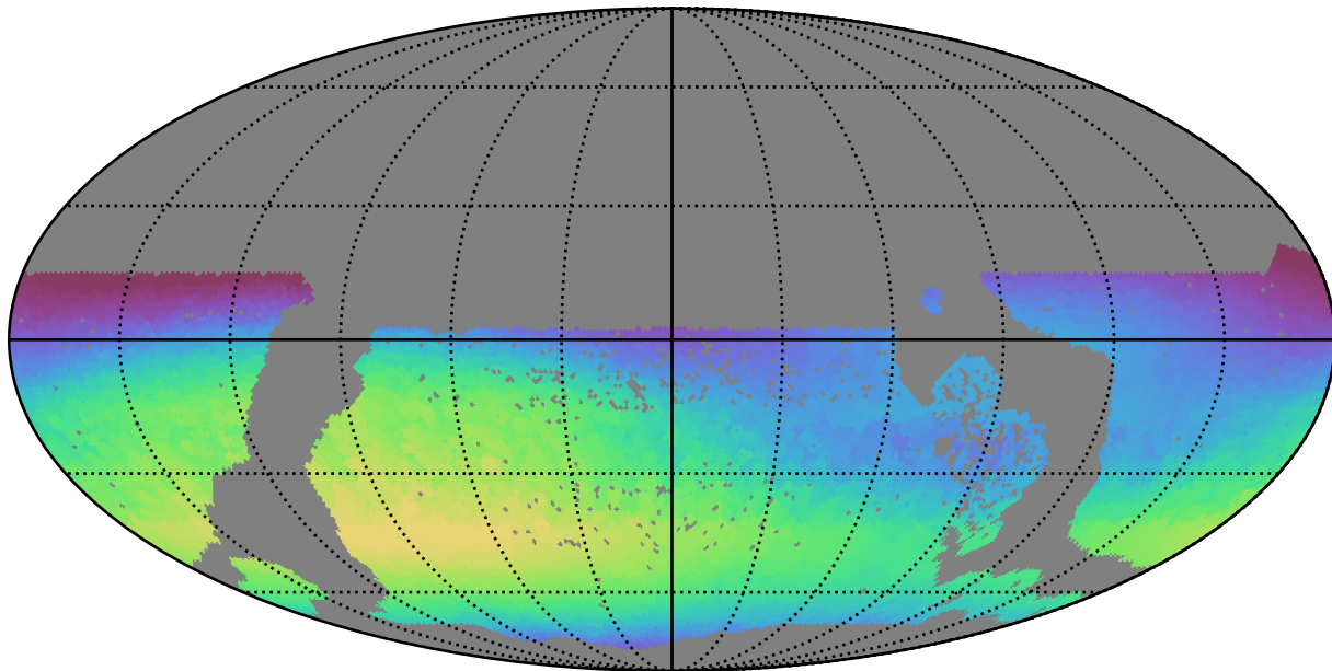
too_100_4v3.4_10yrs WFD all bands: Max skyBrightness
