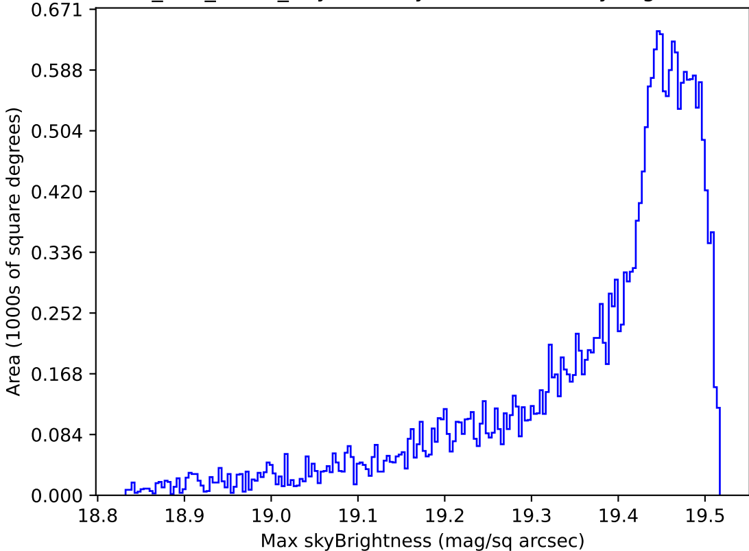
too_100_4v3.4_10yrs All sky z band: Max skyBrightness
