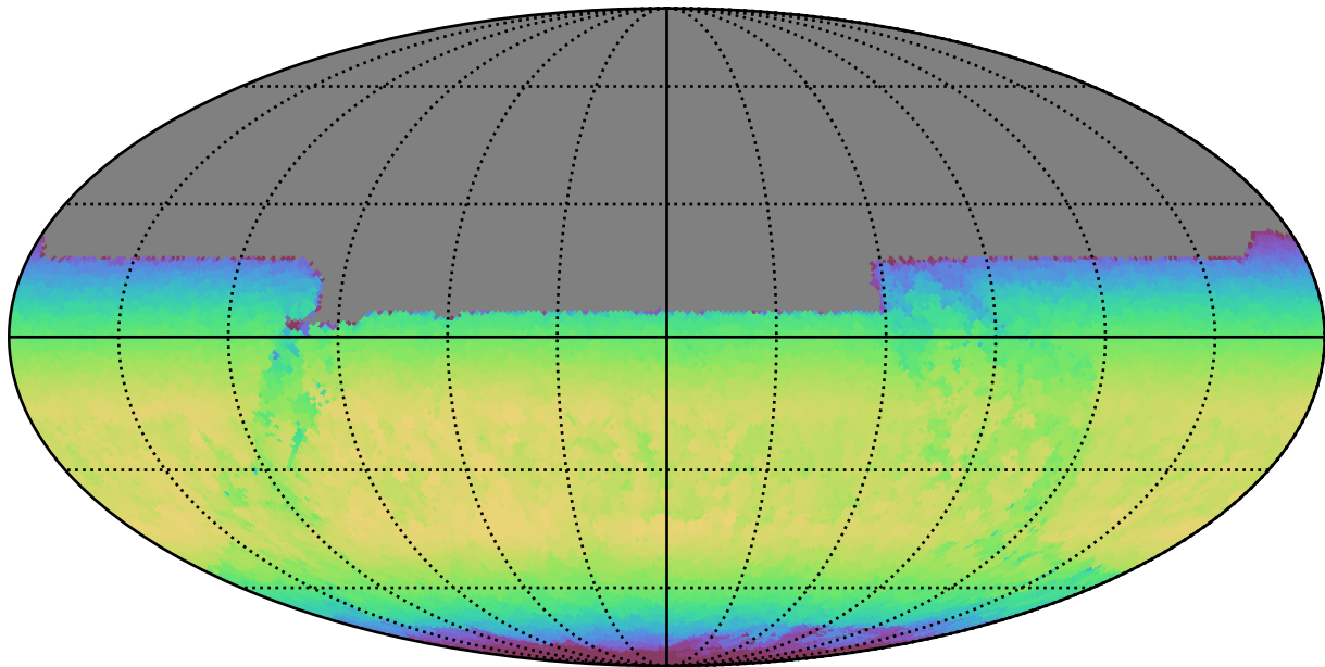
too_100_4v3.4_10yrs All sky y band: Max skyBrightness
