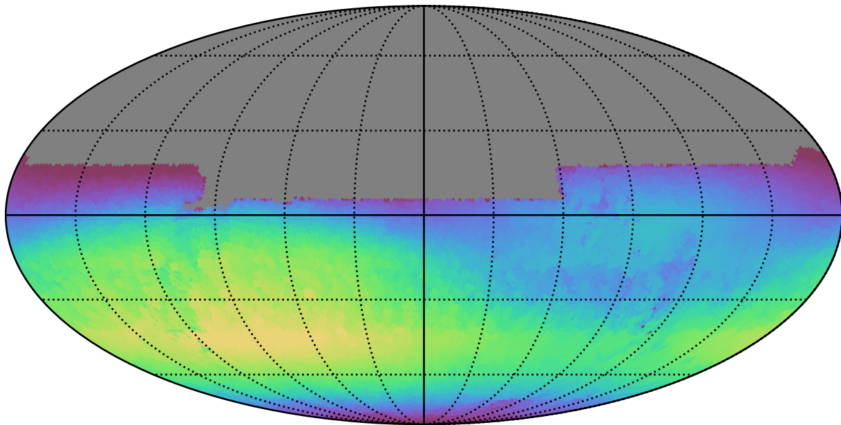
too_100_4v3.4_10yrs All sky u band: Max skyBrightness
