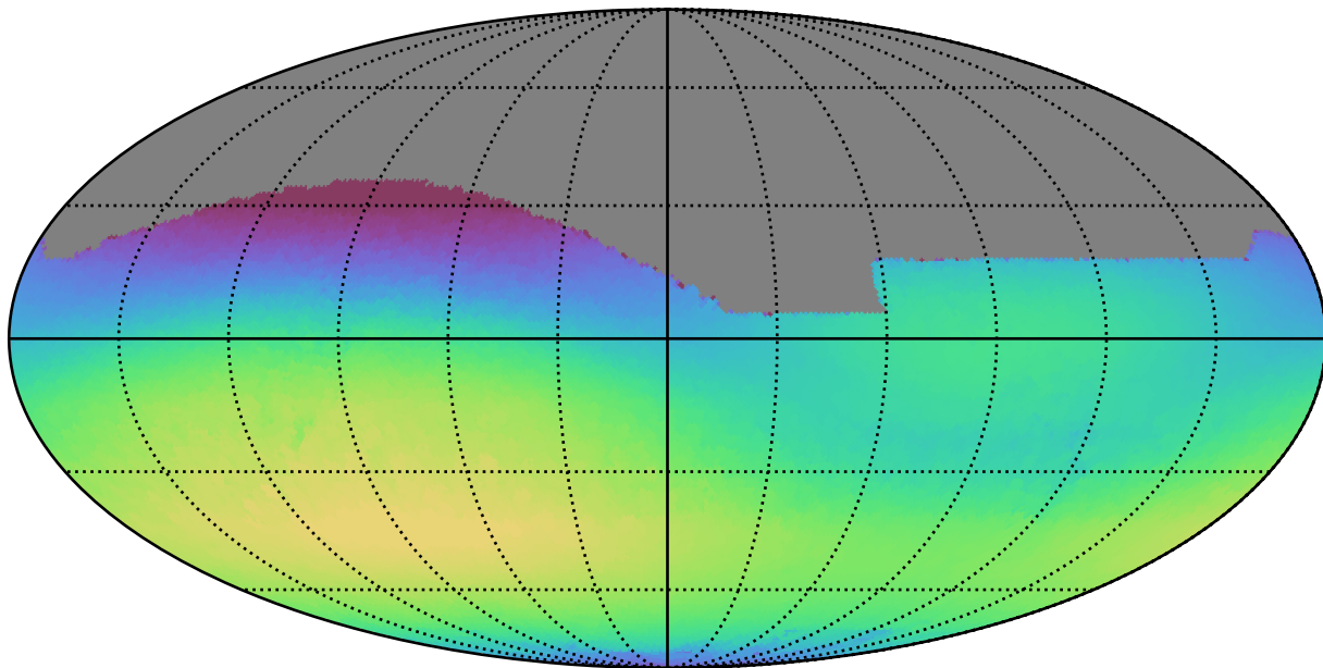
too_100_4v3.4_10yrs All sky r band: Max skyBrightness
