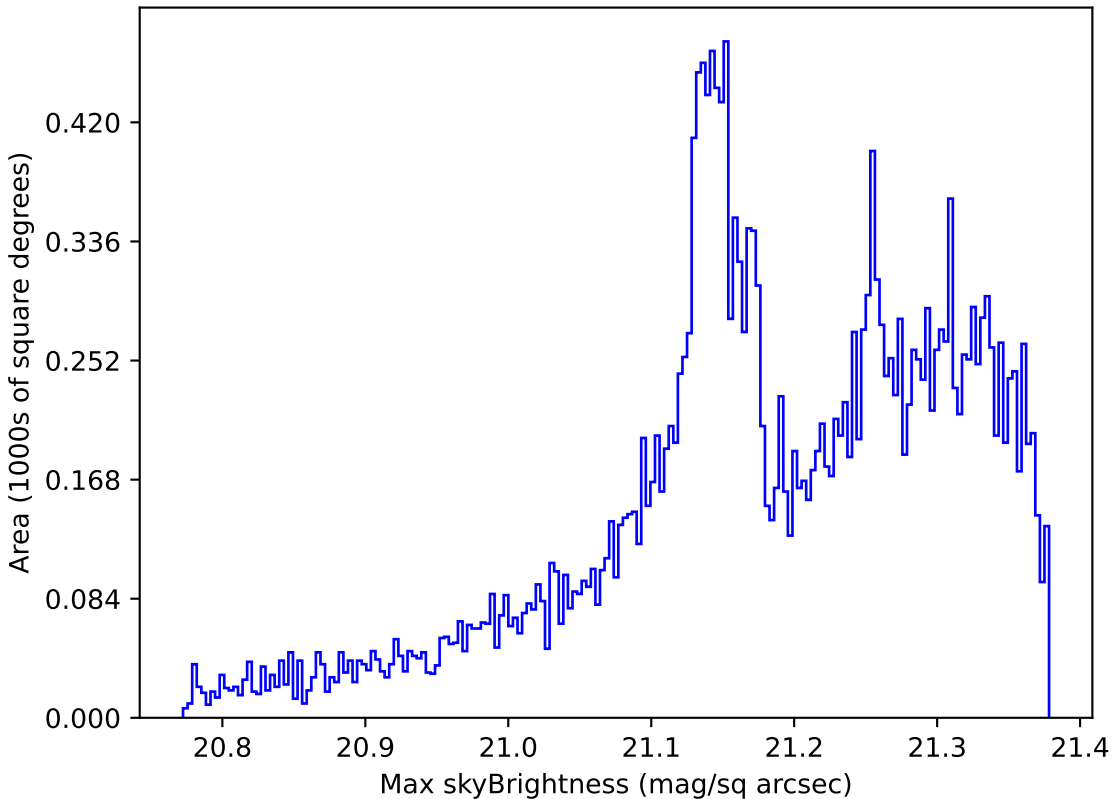
too_100_4v3.4_10yrs All sky r band: Max skyBrightness
