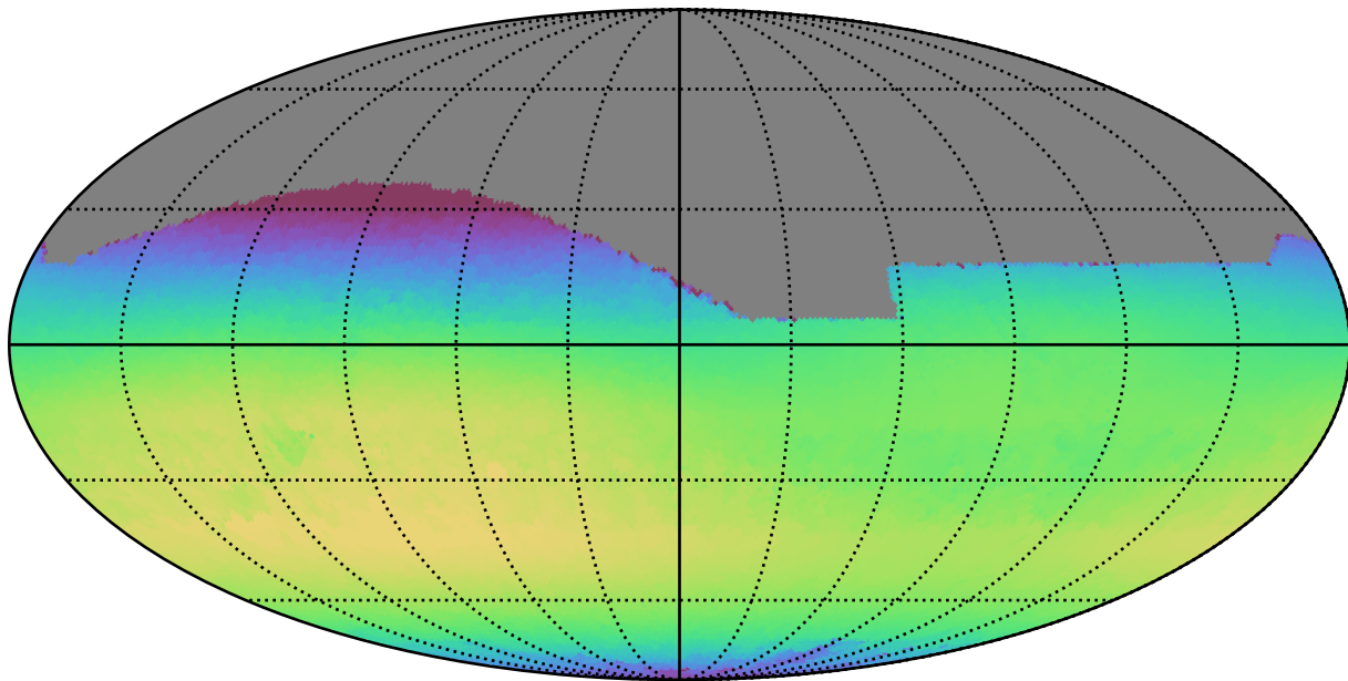
too_100_4v3.4_10yrs All sky i band: Max skyBrightness
