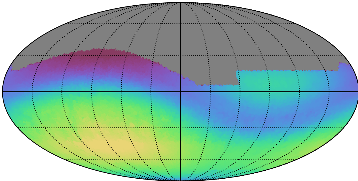
too_100_4v3.4_10yrs All sky g band: Max skyBrightness
