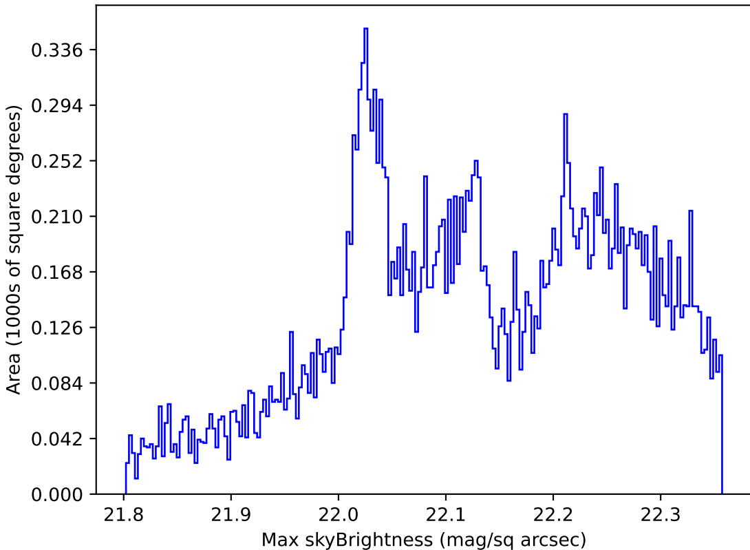
too_100_4v3.4_10yrs All sky g band: Max skyBrightness
