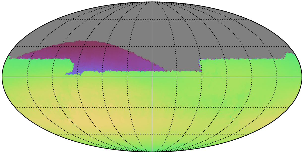
too_100_4v3.4_10yrs All sky all bands: Max skyBrightness
