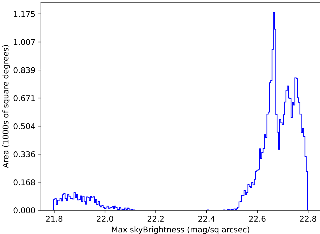
too_100_4v3.4_10yrs All sky all bands: Max skyBrightness
