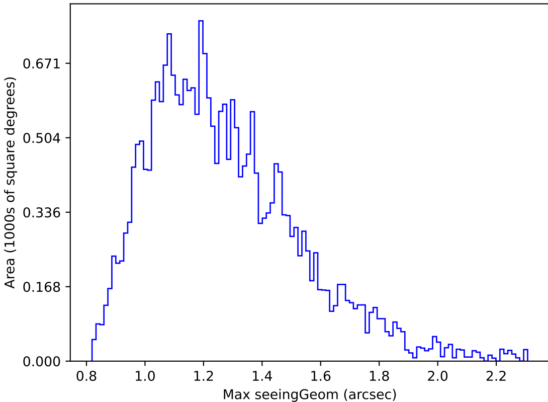
too_100_4v3.4_10yrs Yr 1 z band: Max seeingGeom
