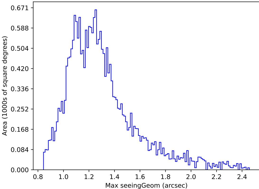
too_100_4v3.4_10yrs Yr 1 y band: Max seeingGeom
