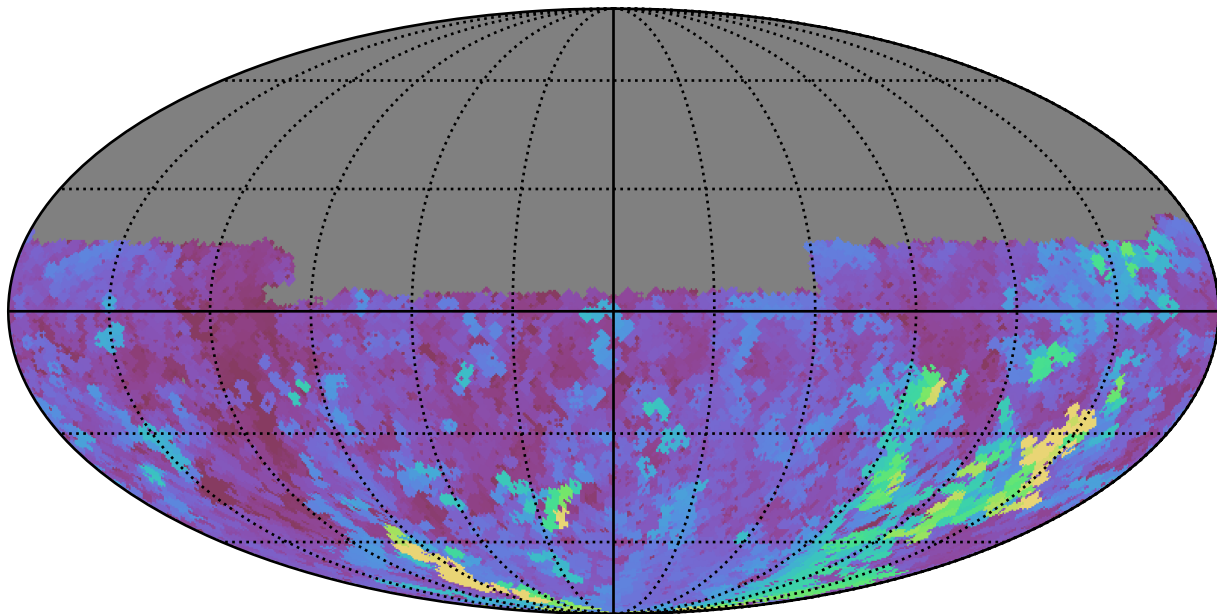
too_100_4v3.4_10yrs Yr 1 u band: Max seeingGeom
