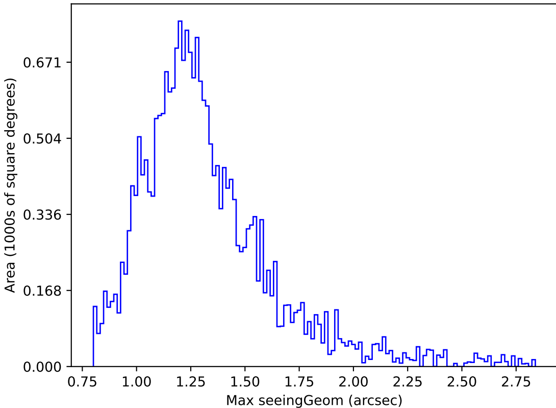
too_100_4v3.4_10yrs Yr 1 u band: Max seeingGeom
