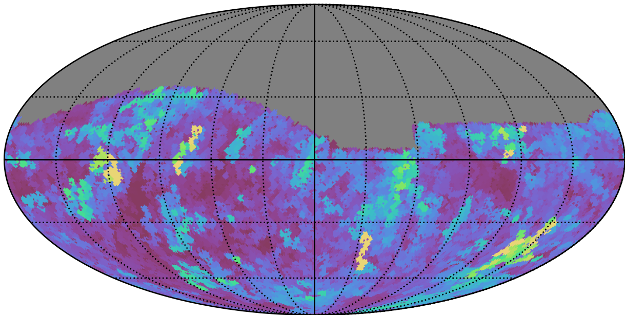
too_100_4v3.4_10yrs Yr 1 r band: Max seeingGeom
