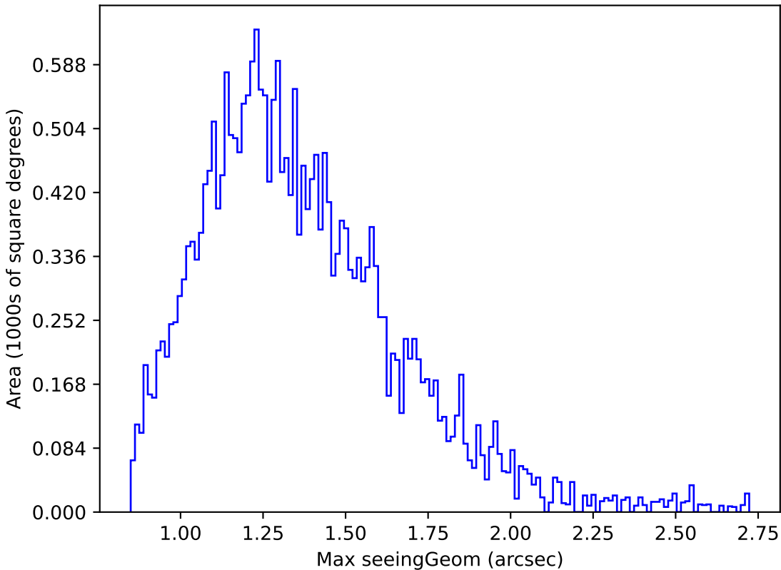
too_100_4v3.4_10yrs Yr 1 r band: Max seeingGeom
