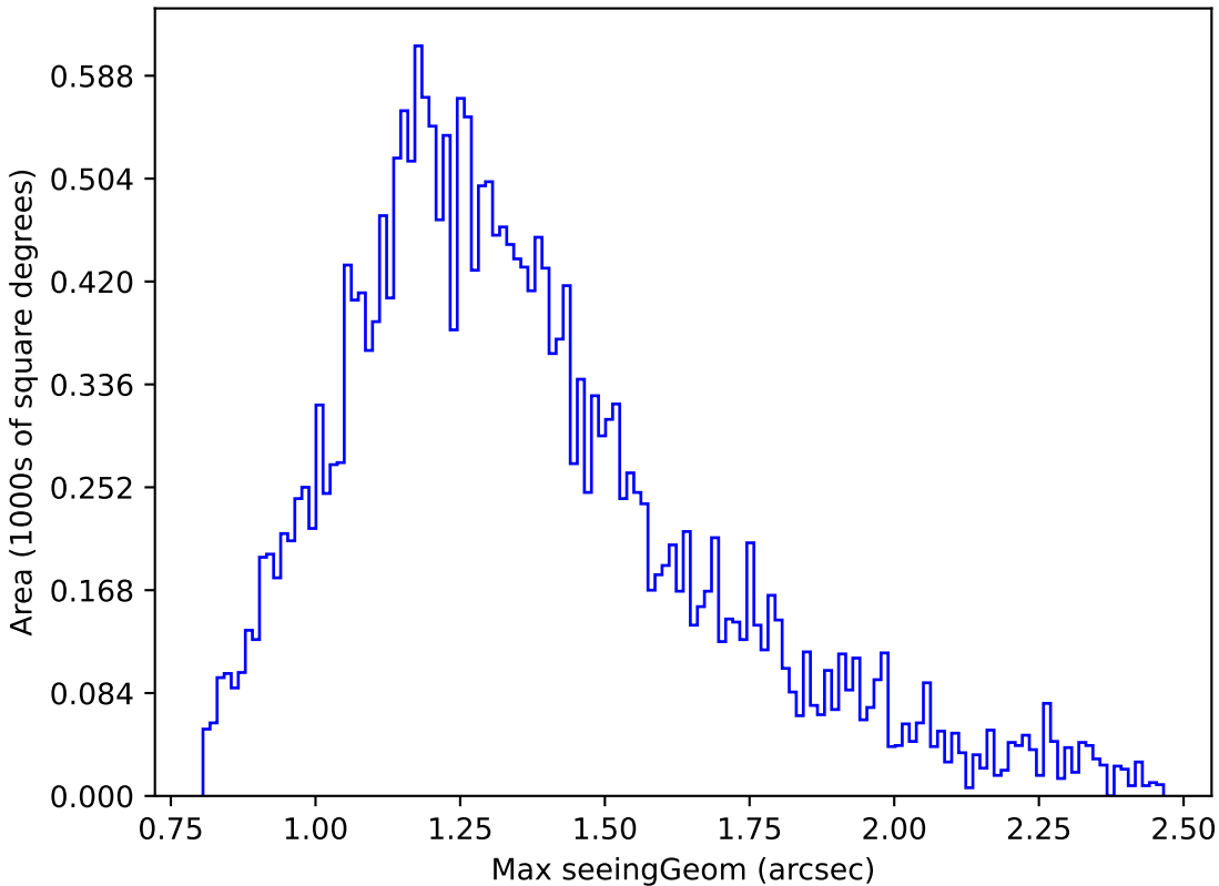
too_100_4v3.4_10yrs Yr 1 g band: Max seeingGeom
