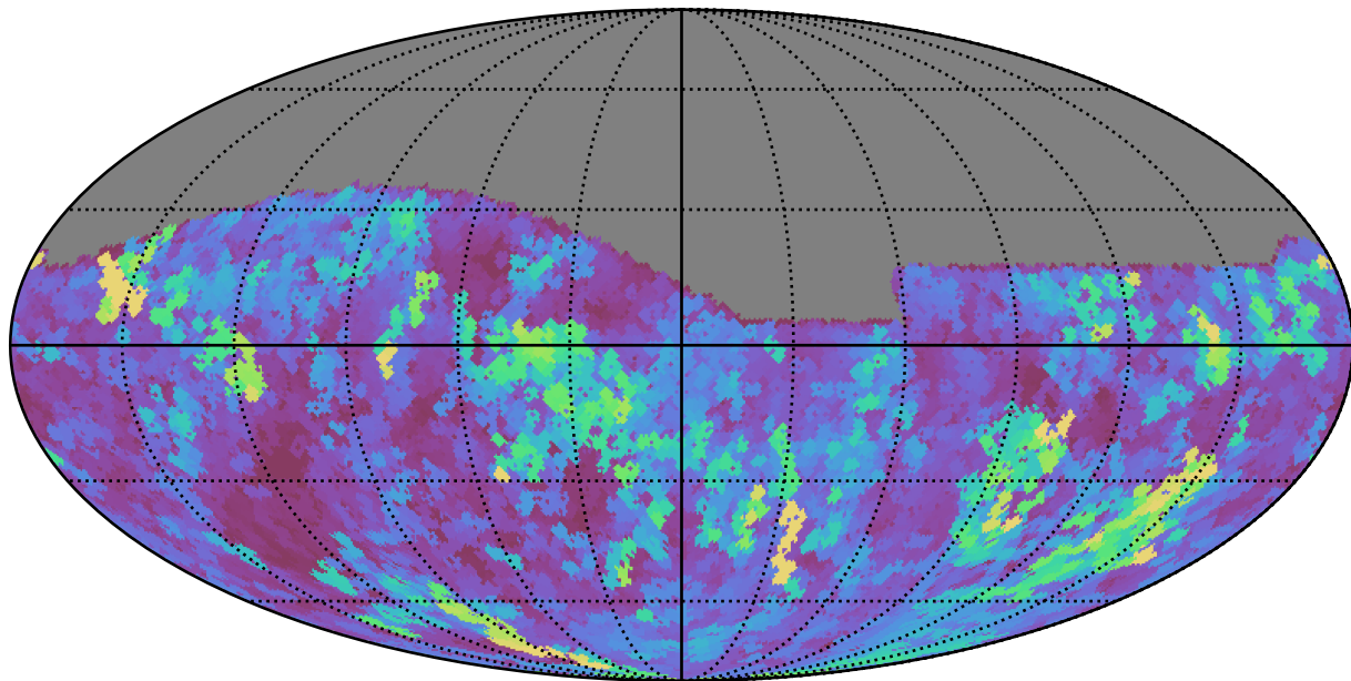
too_100_4v3.4_10yrs Yr 1 all bands: Max seeingGeom
