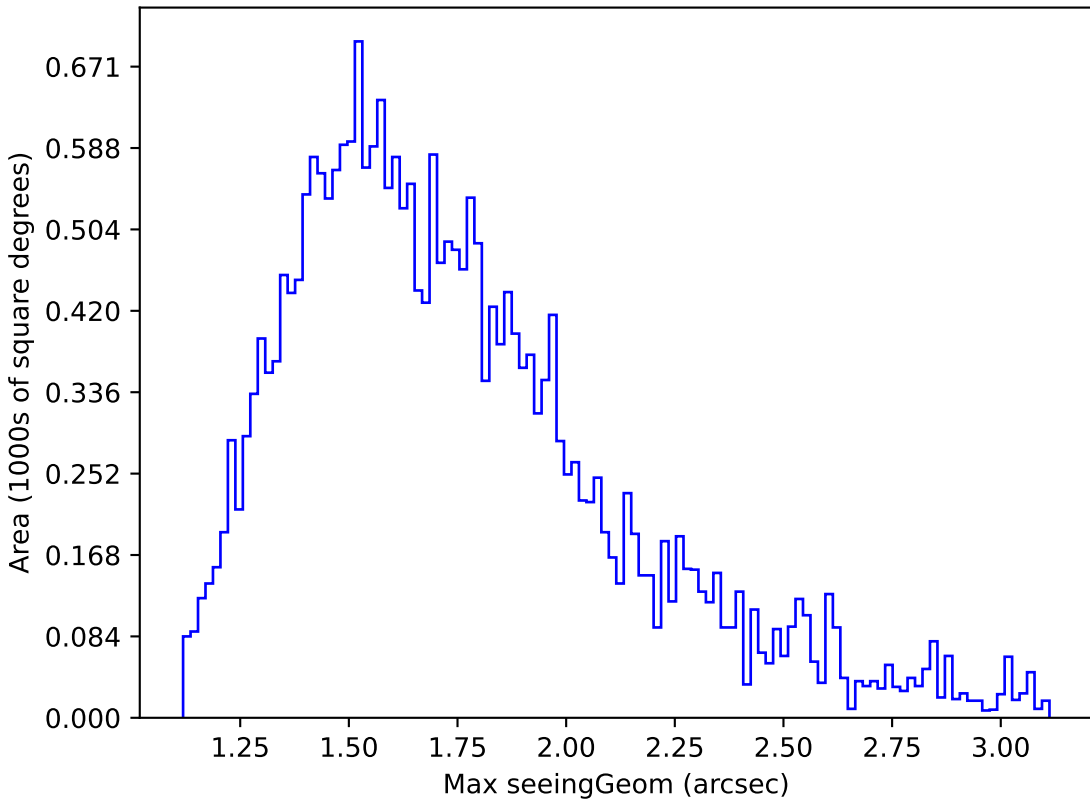
too_100_4v3.4_10yrs Yr 1 all bands: Max seeingGeom
