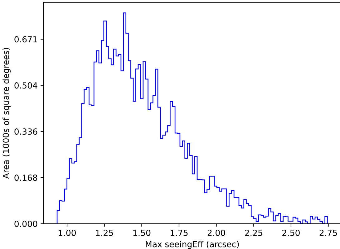
too_100_4v3.4_10yrs Yr 1 z band: Max seeingEff
