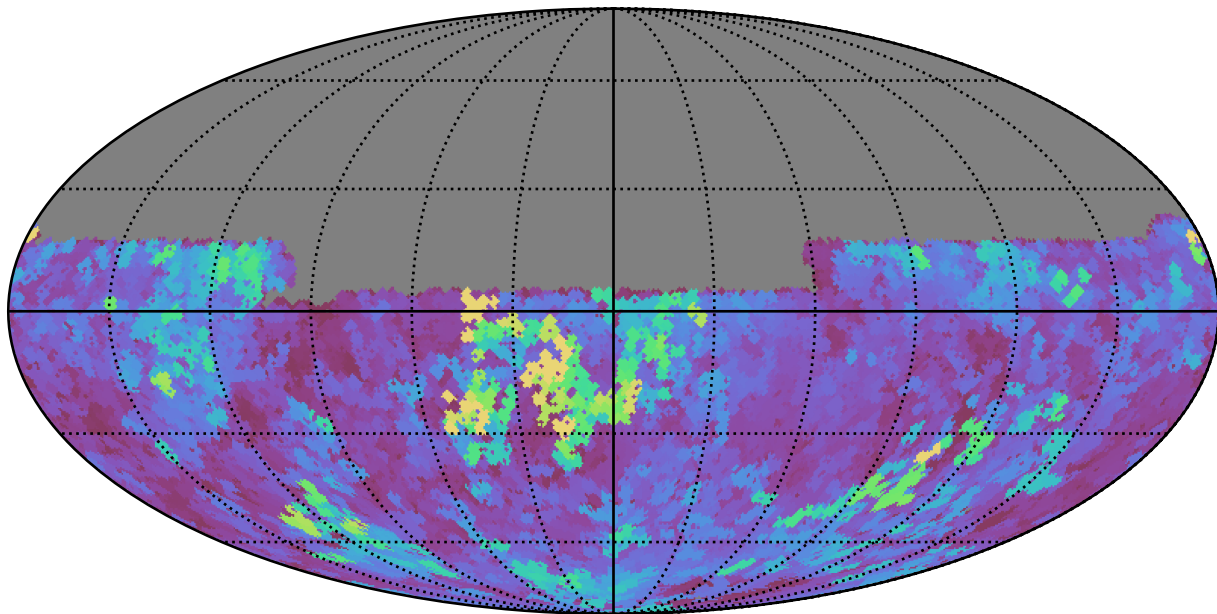
too_100_4v3.4_10yrs Yr 1 y band: Max seeingEff
