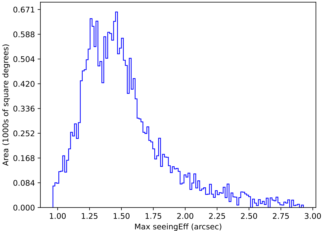
too_100_4v3.4_10yrs Yr 1 y band: Max seeingEff
