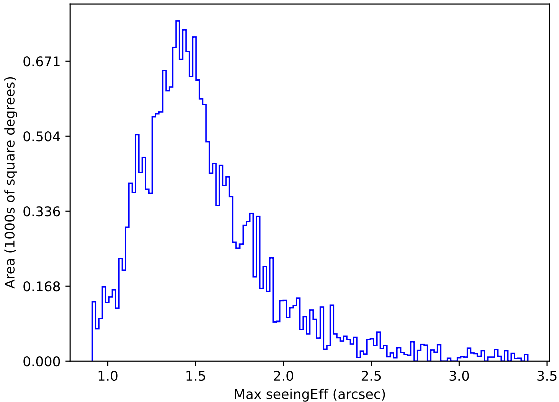
too_100_4v3.4_10yrs Yr 1 u band: Max seeingEff
