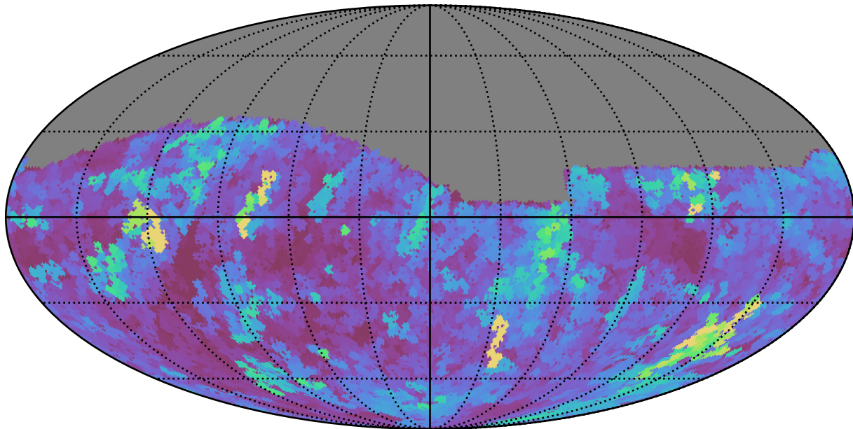
too_100_4v3.4_10yrs Yr 1 r band: Max seeingEff
