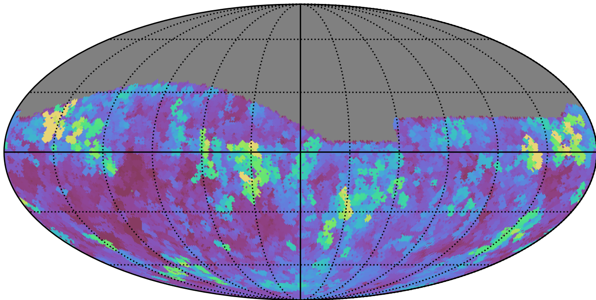
too_100_4v3.4_10yrs Yr 1 i band: Max seeingEff
