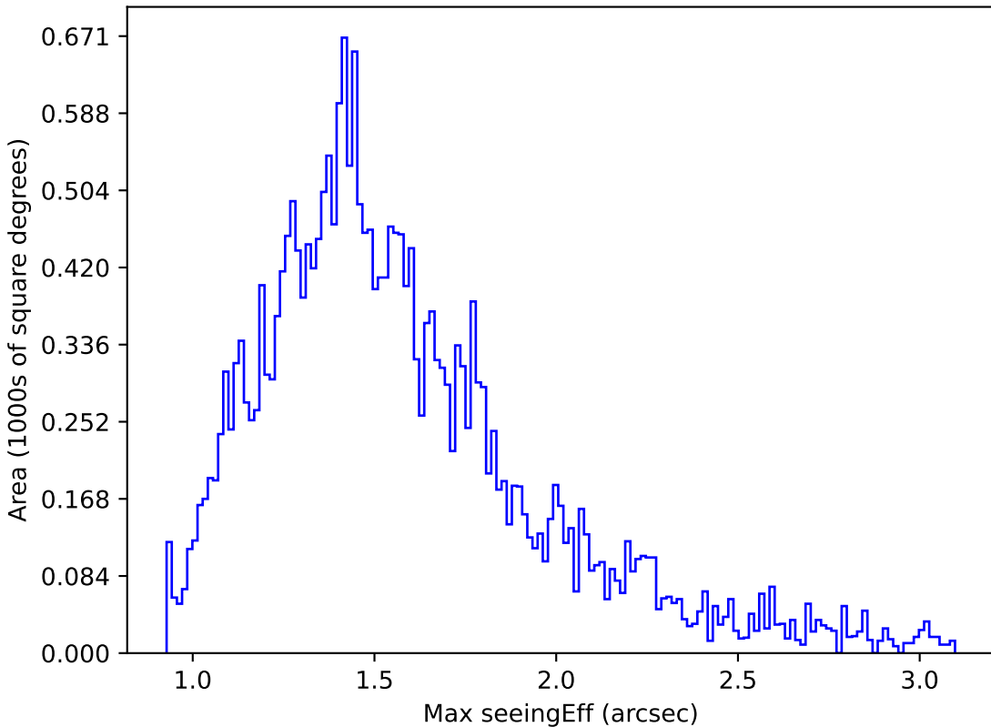
too_100_4v3.4_10yrs Yr 1 i band: Max seeingEff
