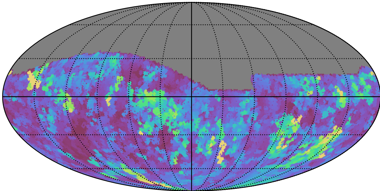
too_100_4v3.4_10yrs Yr 1 all bands: Max seeingEff
