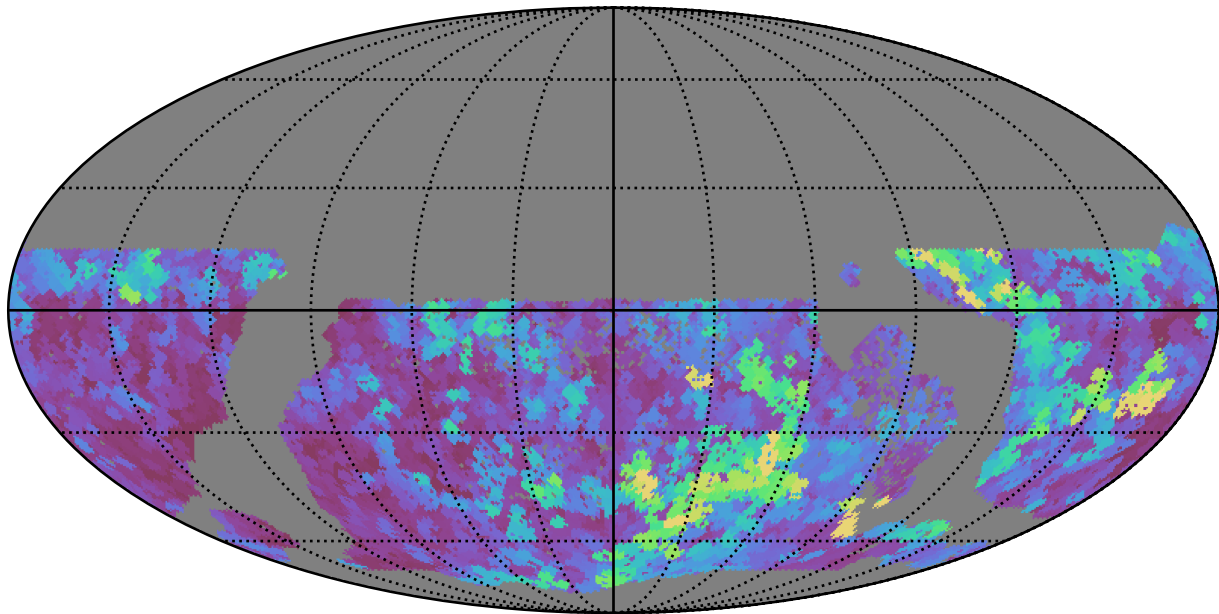
too_100_4v3.4_10yrs WFD z band: Max seeingEff
