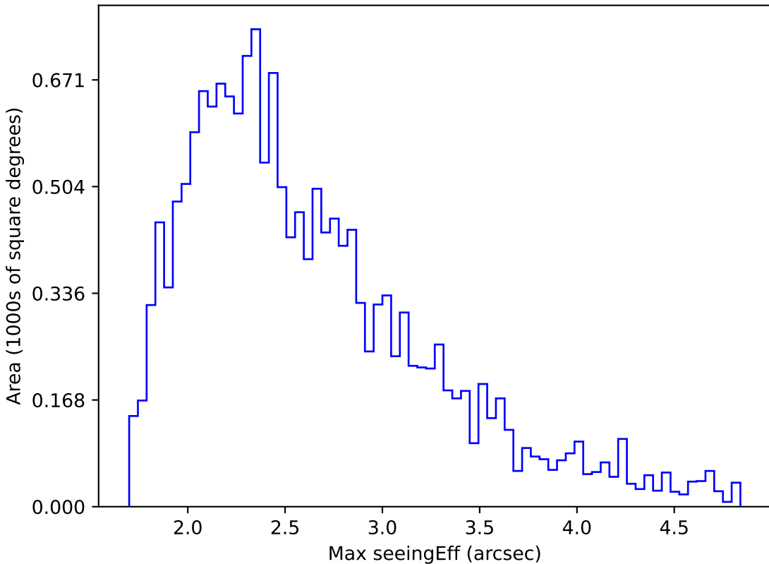
too_100_4v3.4_10yrs WFD z band: Max seeingEff
