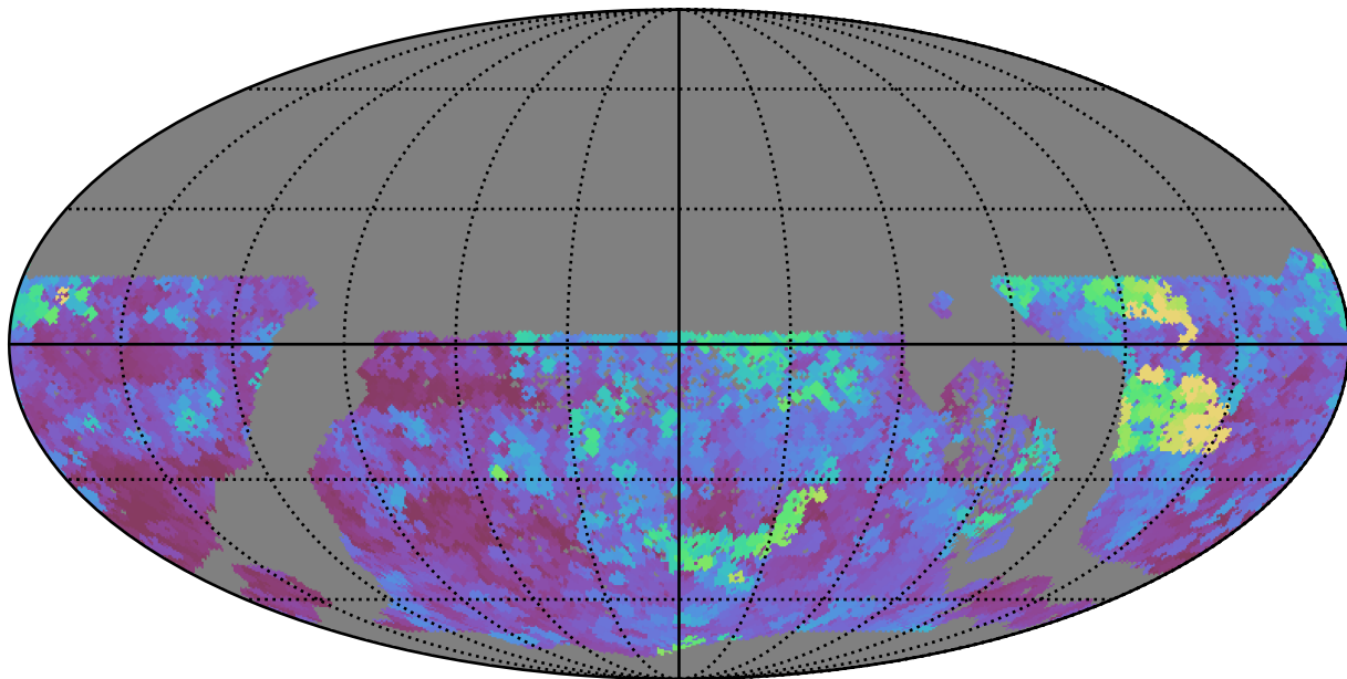
too_100_4v3.4_10yrs WFD y band: Max seeingEff
