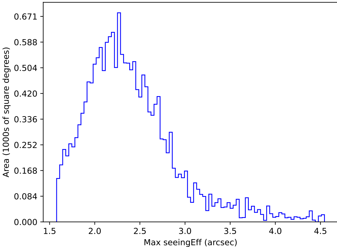
too_100_4v3.4_10yrs WFD y band: Max seeingEff
