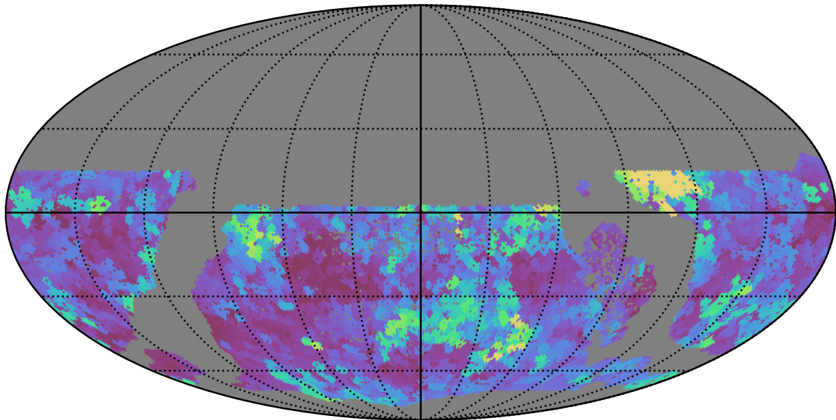
too_100_4v3.4_10yrs WFD u band: Max seeingEff
