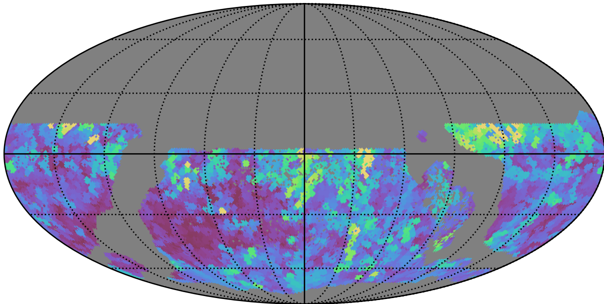
too_100_4v3.4_10yrs WFD r band: Max seeingEff
