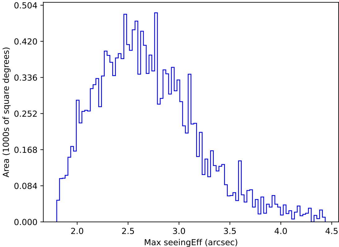
too_100_4v3.4_10yrs WFD r band: Max seeingEff
