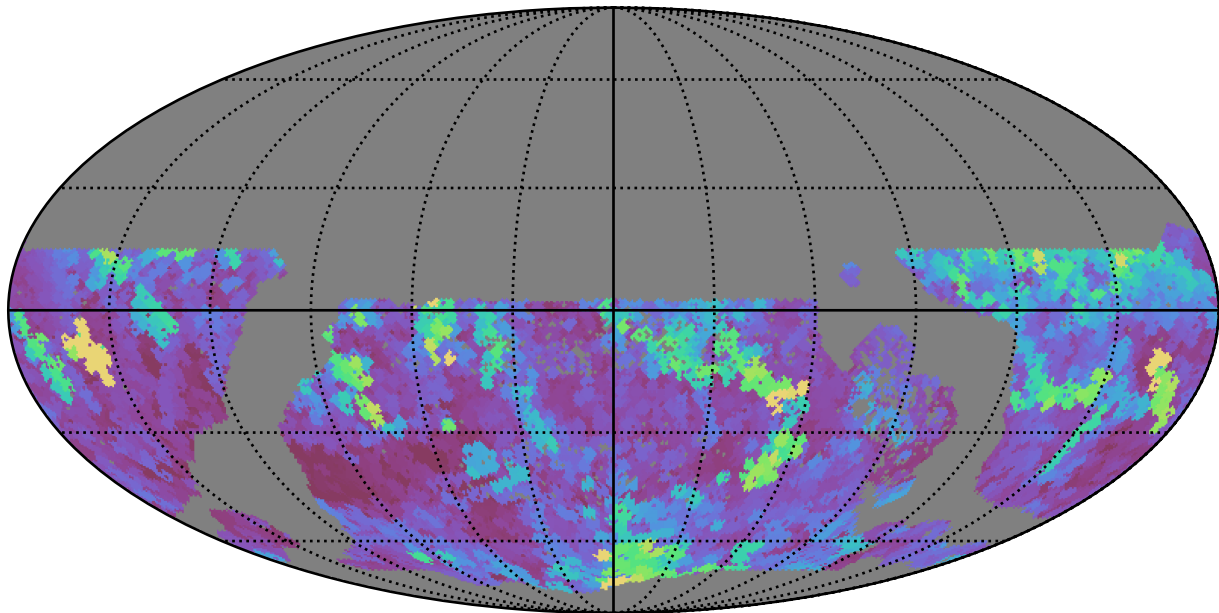
too_100_4v3.4_10yrs WFD i band: Max seeingEff
