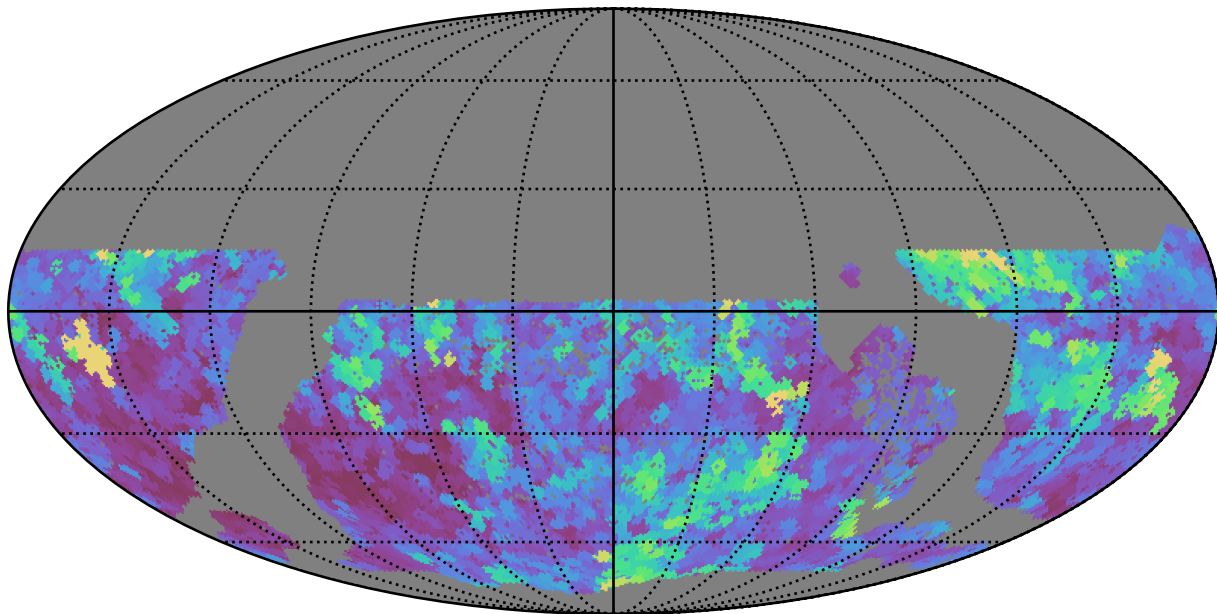
too_100_4v3.4_10yrs WFD all bands: Max seeingEff
