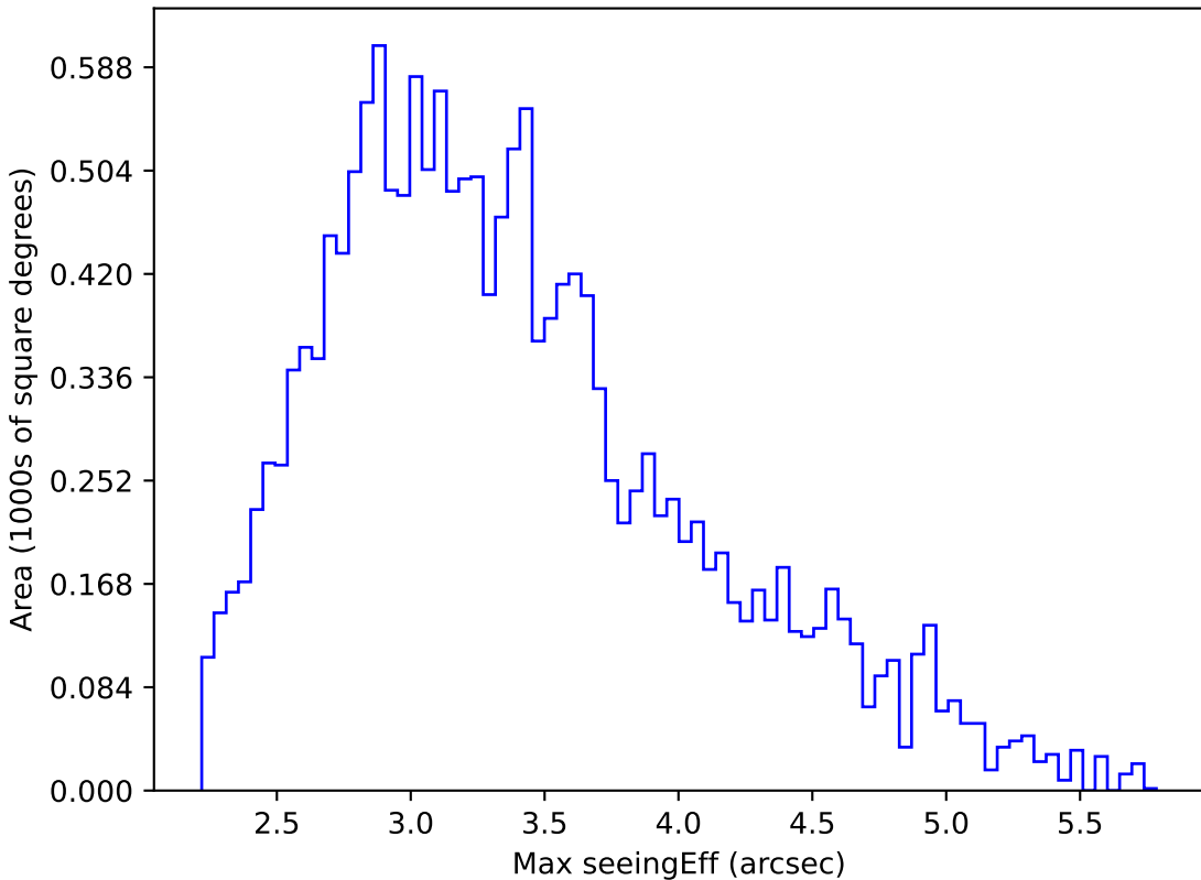
too_100_4v3.4_10yrs WFD all bands: Max seeingEff
