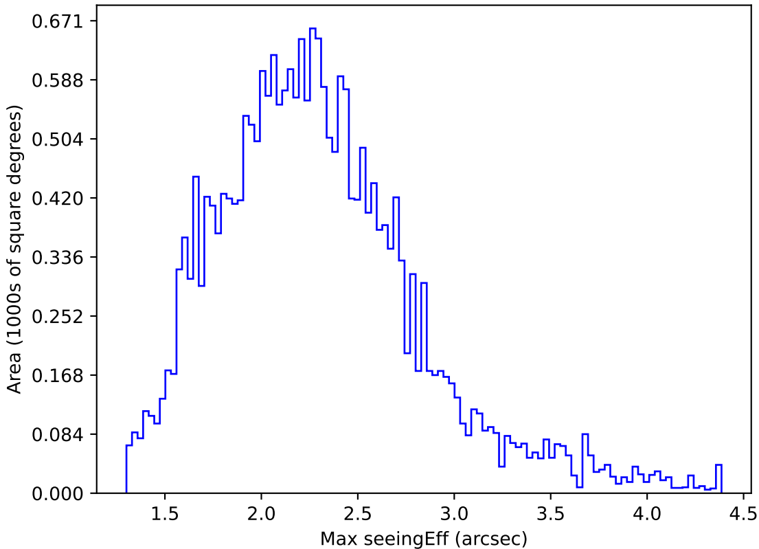
too_100_4v3.4_10yrs All sky y band: Max seeingEff
