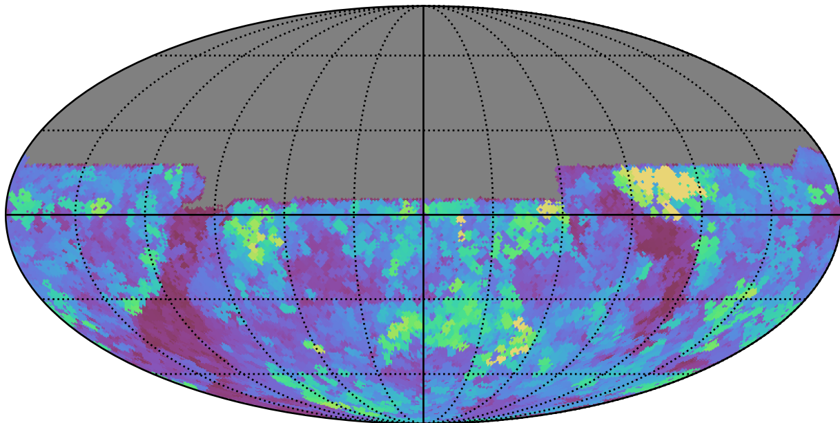
too_100_4v3.4_10yrs All sky u band: Max seeingEff
