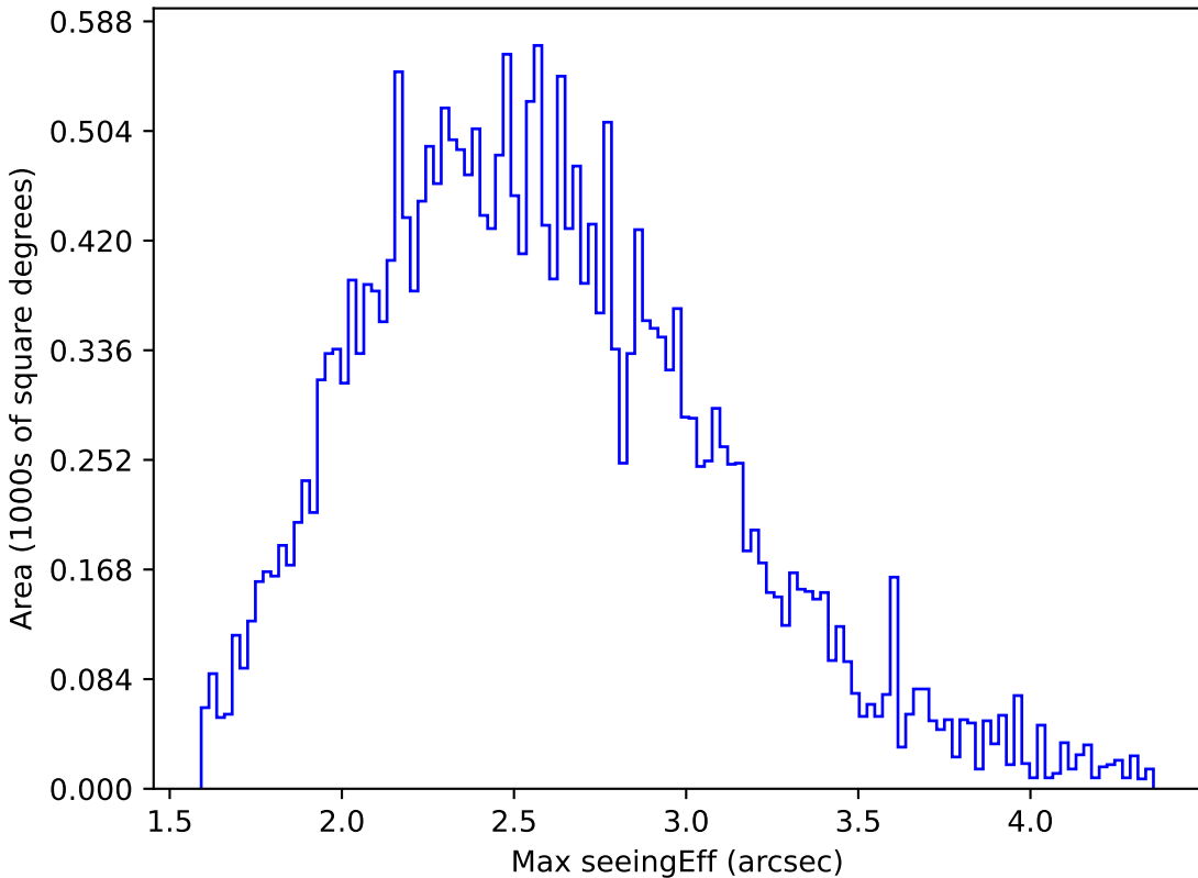
too_100_4v3.4_10yrs All sky r band: Max seeingEff
