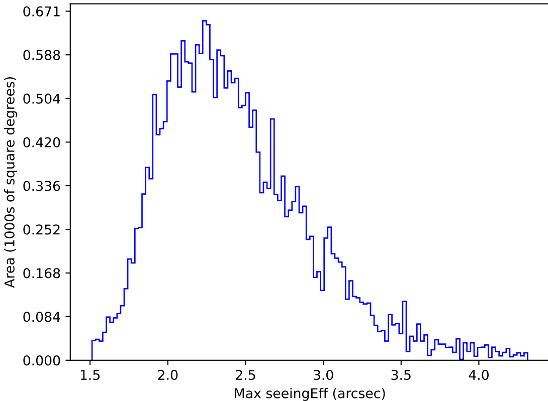
too_100_4v3.4_10yrs All sky g band: Max seeingEff
