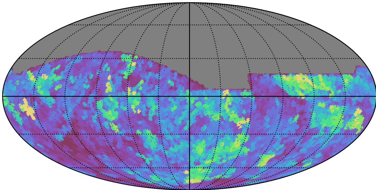
too_100_4v3.4_10yrs All sky all bands: Max seeingEff
