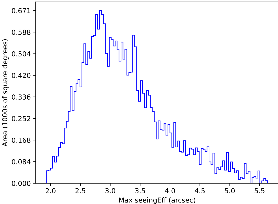
too_100_4v3.4_10yrs All sky all bands: Max seeingEff
