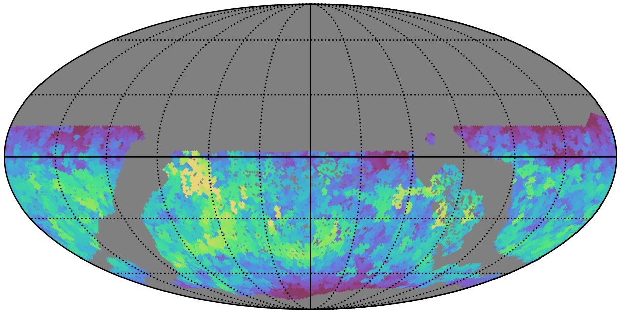
too_100_4v3.4_10yrs WFD z band: Max saturation_mag
