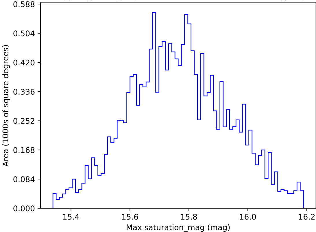
too_100_4v3.4_10yrs WFD r band: Max saturation_mag
