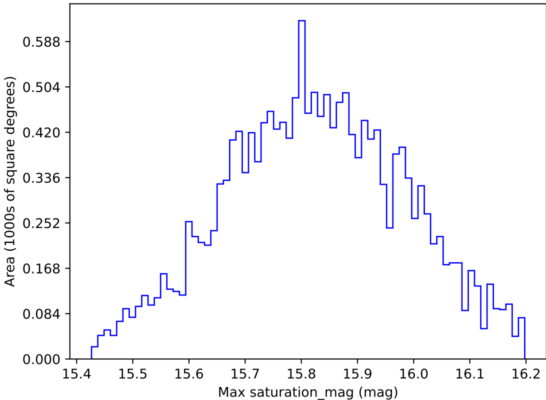
too_100_4v3.4_10yrs WFD all bands: Max saturation_mag
