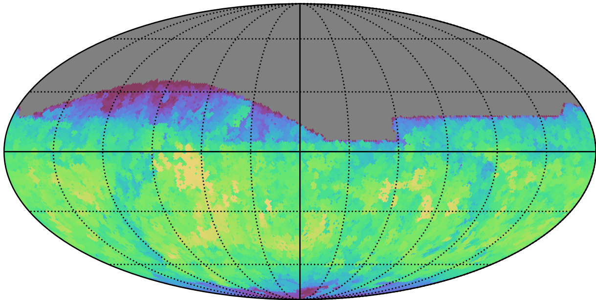
too_100_4v3.4_10yrs All sky z band: Max saturation_mag
