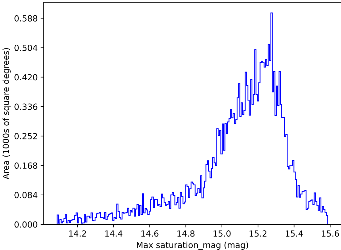
too_100_4v3.4_10yrs All sky z band: Max saturation_mag
